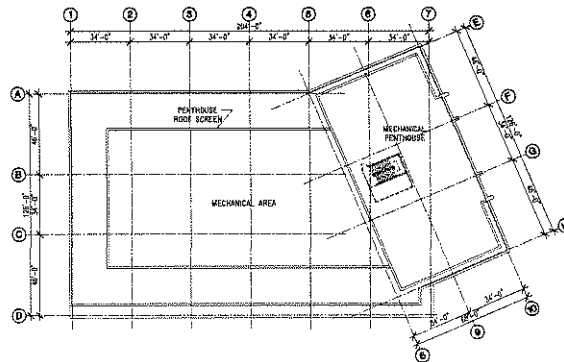
3 ROOF PLAN
