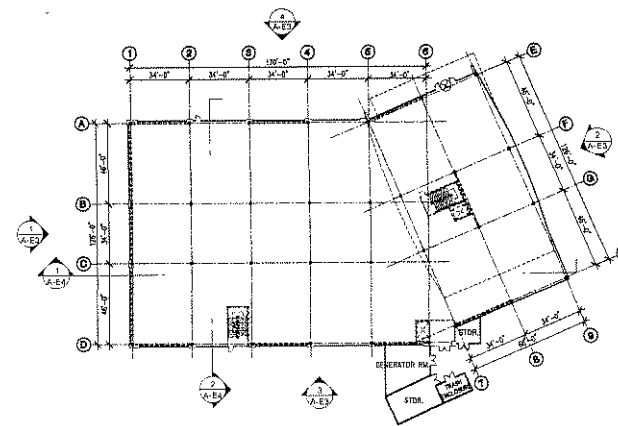
1 FIRST FLOOR PLAN
