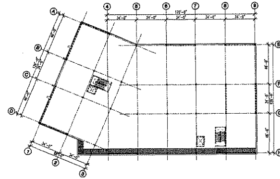
2 4TH FLOOR PLAN
