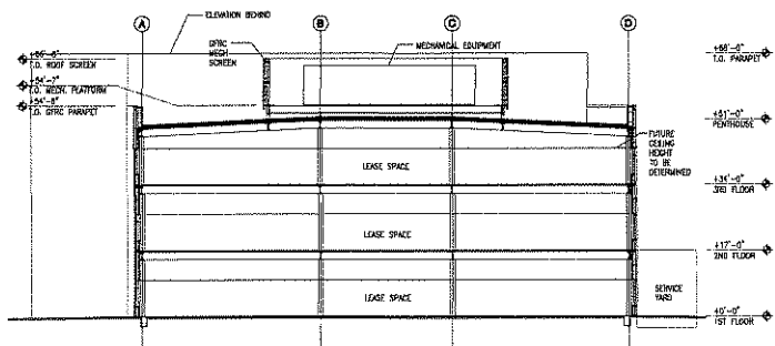
2 BUILDING CROSS SECTION
