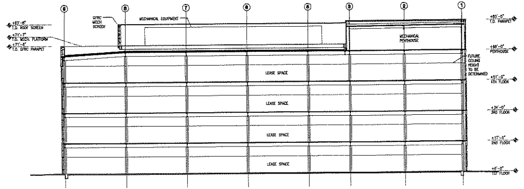
1 BUILDING LONGITUDINAL SECTION
