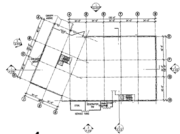
1 FIRST FLOOR PLAN
