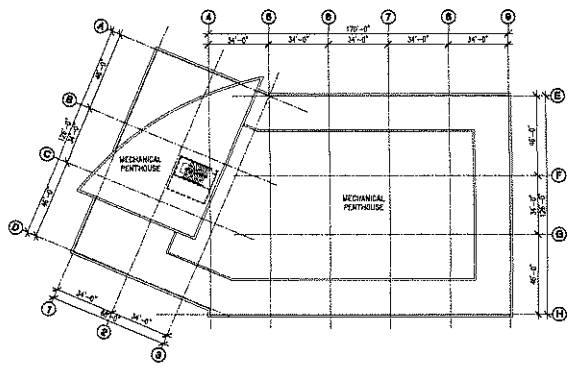
4 ROOF PLAN
