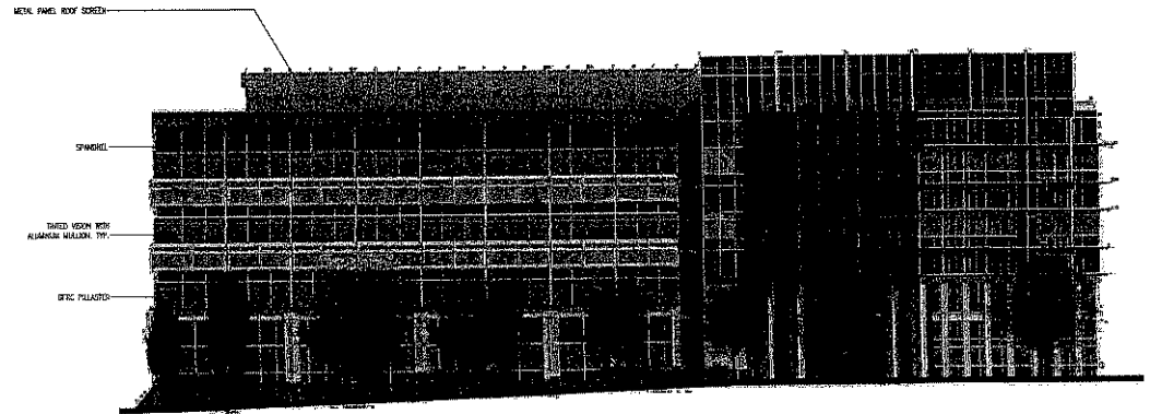
1 WEST ELEVATION
