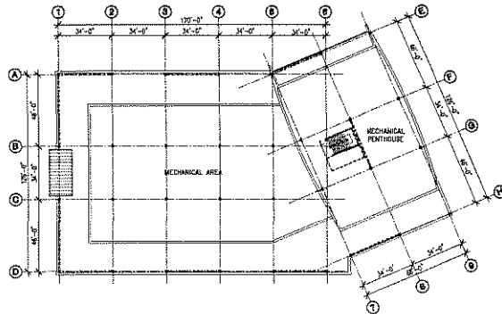
3 ROOF PLAN
