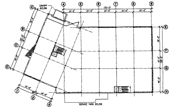
2 SECOND FLOOR PLAN
