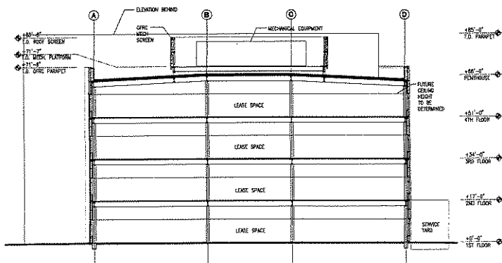
2 BUILDING CROSS SECTION
