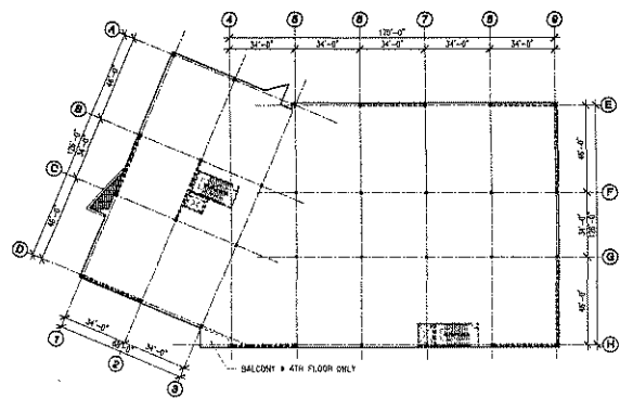
3 THIRD & FOURTH FLOOR PLAN
