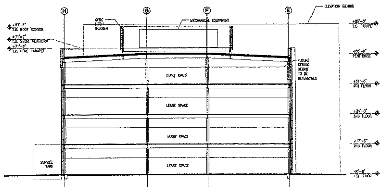
2 BUILDING CROSS SECTION
