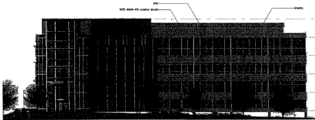
3 SOUTH ELEVATION
