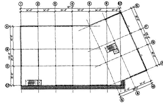
2 FOURTH FLOOR PLAN
