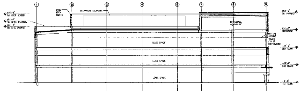
1 BUILDING LONGITUDINAL SECTION
