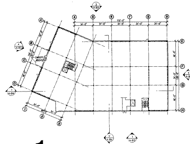
1 1ST, 2ND & 3RD FLOOR PLAN
