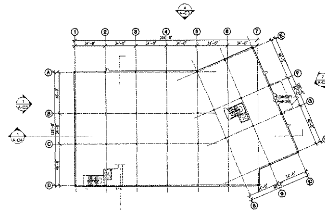
2 FOURTH FLOOR PLAN
