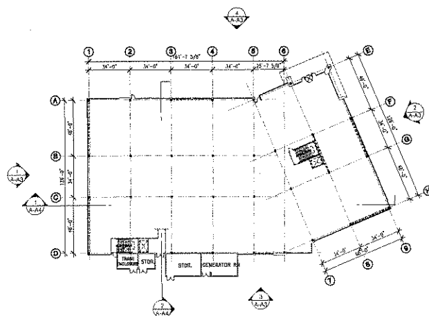
1 FIRST FLOOR PLAN
